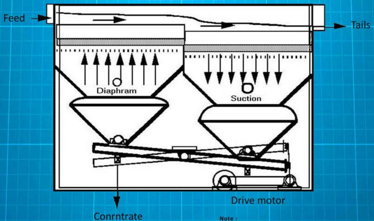
Figure 1. selection of modern placer jig
